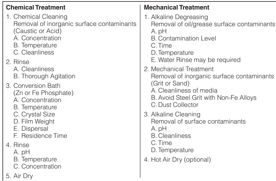
Chart 2 - Elastomer Bonding Flowchart
