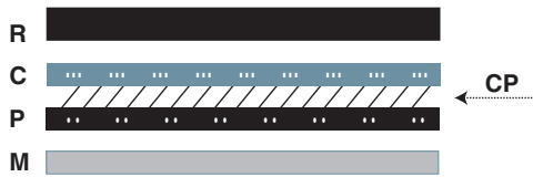
Figure 4 – Cement-Primer Failure
